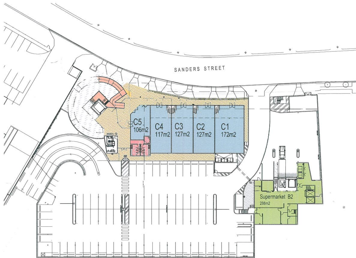
BASEMENT 02 LEVEL
